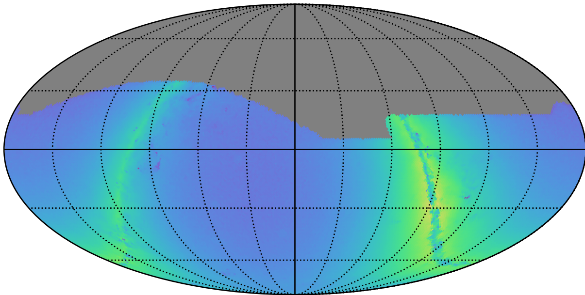
baseline_v3.3_10yrs g: Nstars_no_crowding
