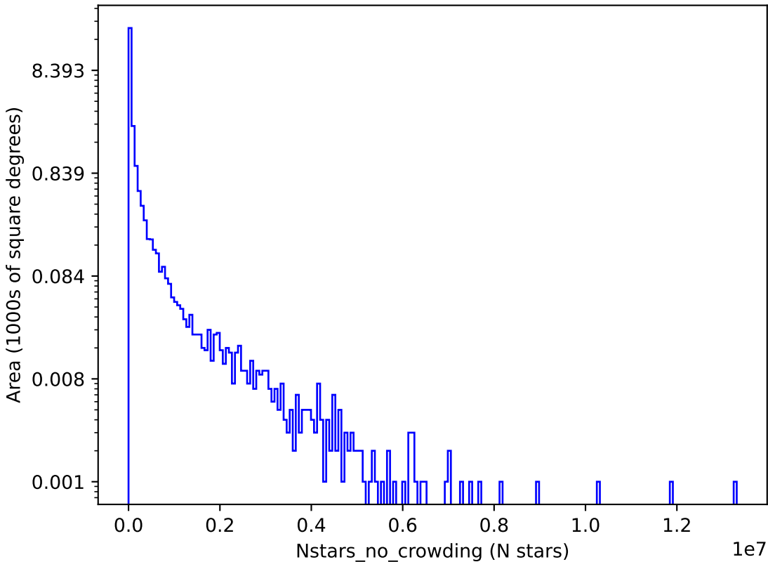
baseline_v3.3_10yrs g: Nstars_no_crowding
