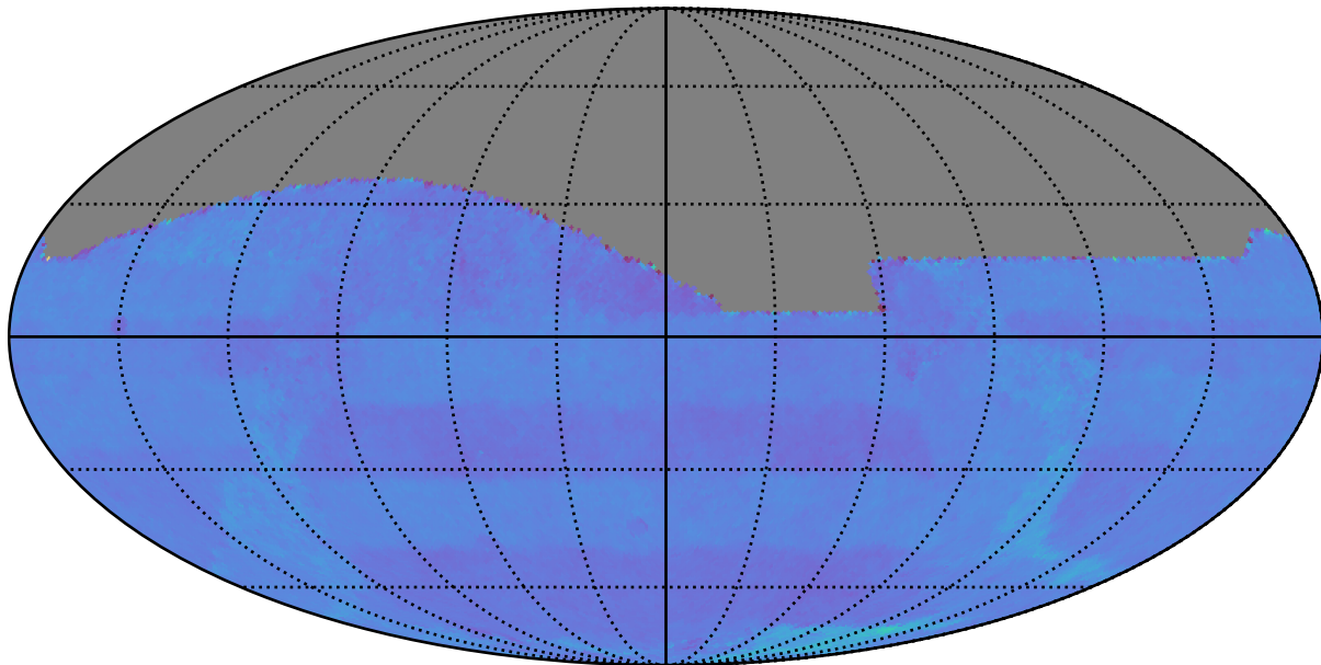
baseline_v3.3_10yrs : Normalized Proper Motion Uncert @ 24.0
