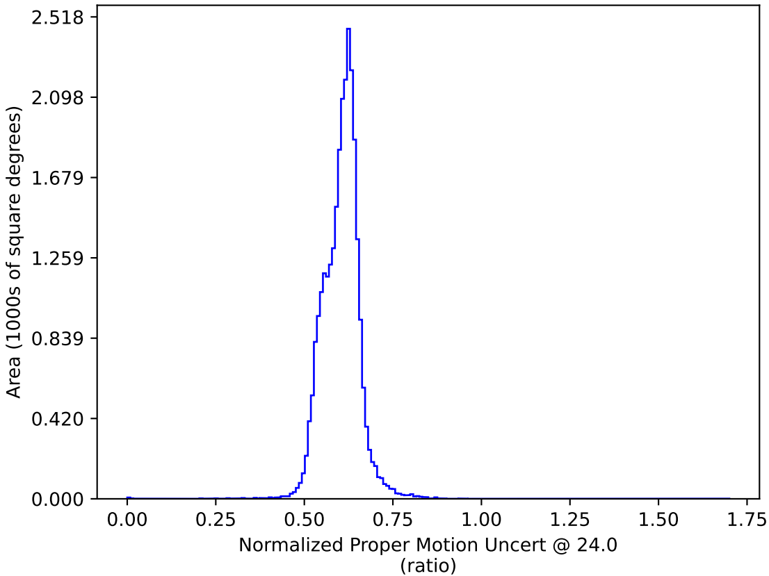
baseline_v3.3_10yrs : Normalized Proper Motion Uncert @ 24.0
