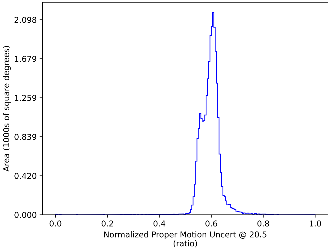
baseline_v3.3_10yrs : Normalized Proper Motion Uncert @ 20.5
