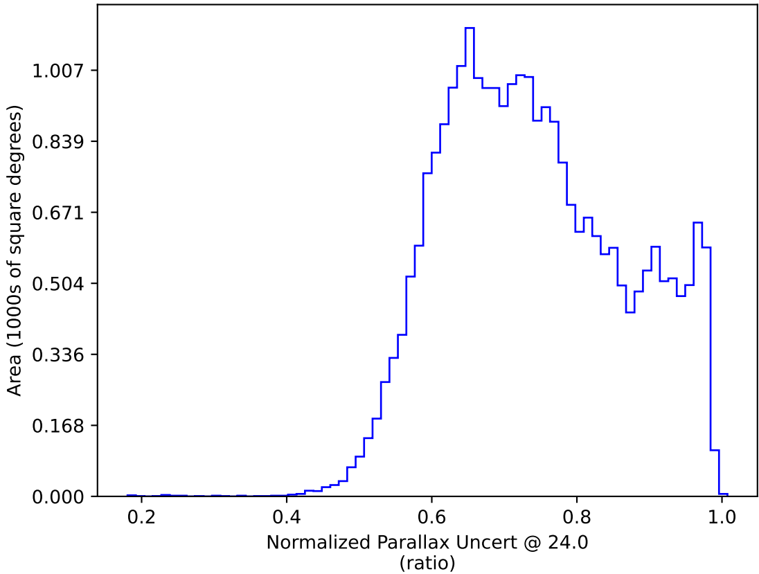
baseline_v3.3_10yrs : Normalized Parallax Uncert @ 24.0
