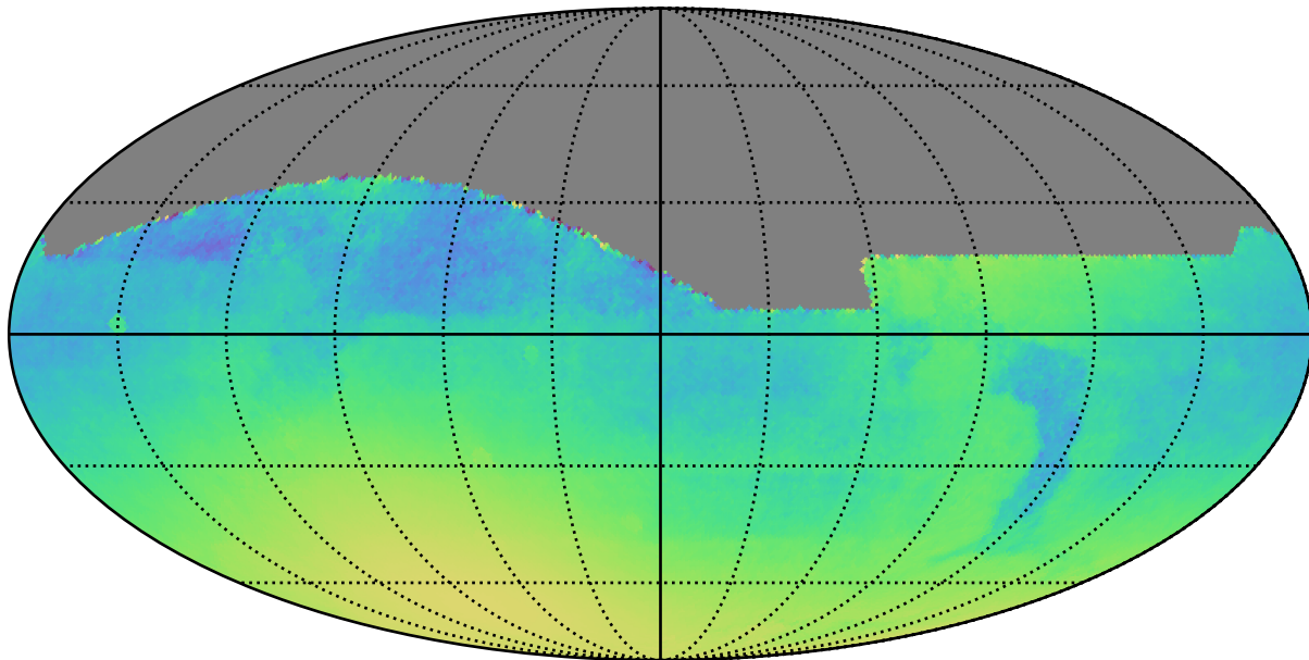
baseline_v3.3_10yrs : Normalized Parallax Uncert @ 22.4
