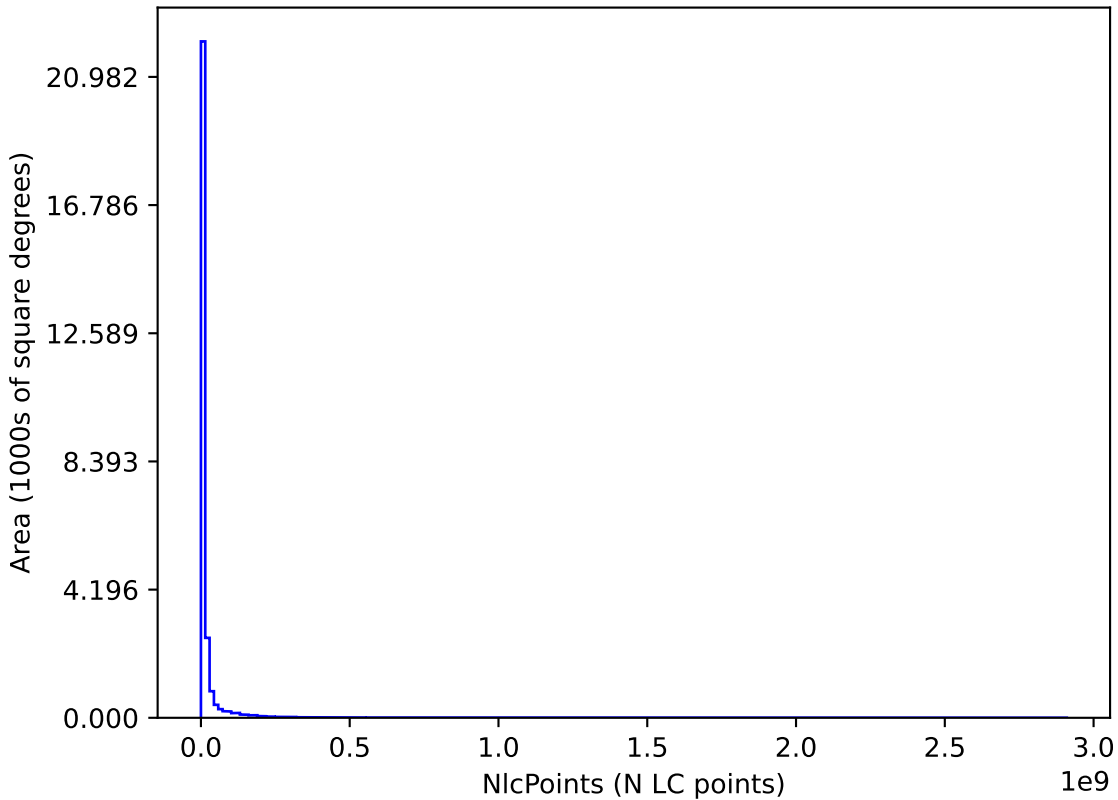
baseline_v3.3_10yrs : NlcPoints
