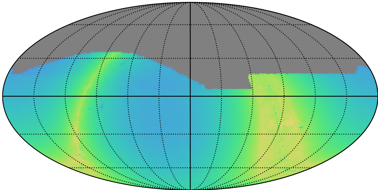
baseline_v3.3_10yrs z: N stars to Precision 0.20
