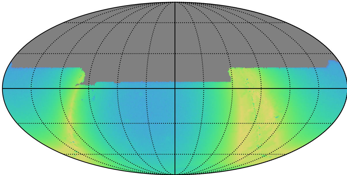
baseline_v3.3_10yrs y: N stars to Precision 0.20
