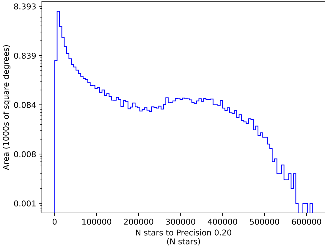
baseline_v3.3_10yrs y: N stars to Precision 0.20
