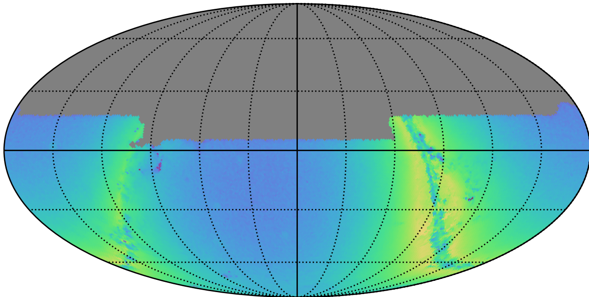
baseline_v3.3_10yrs u: N stars to Precision 0.20
