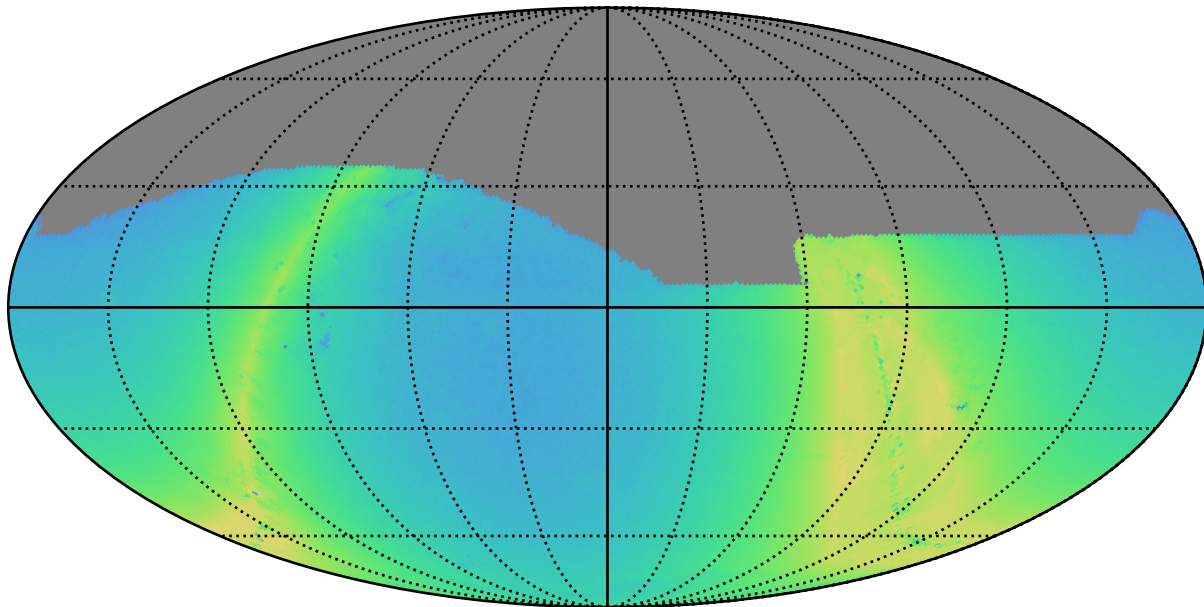
baseline_v3.3_10yrs r: N stars to Precision 0.20
