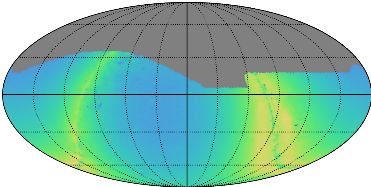
baseline_v3.3_10yrs g: N stars to Precision 0.20
