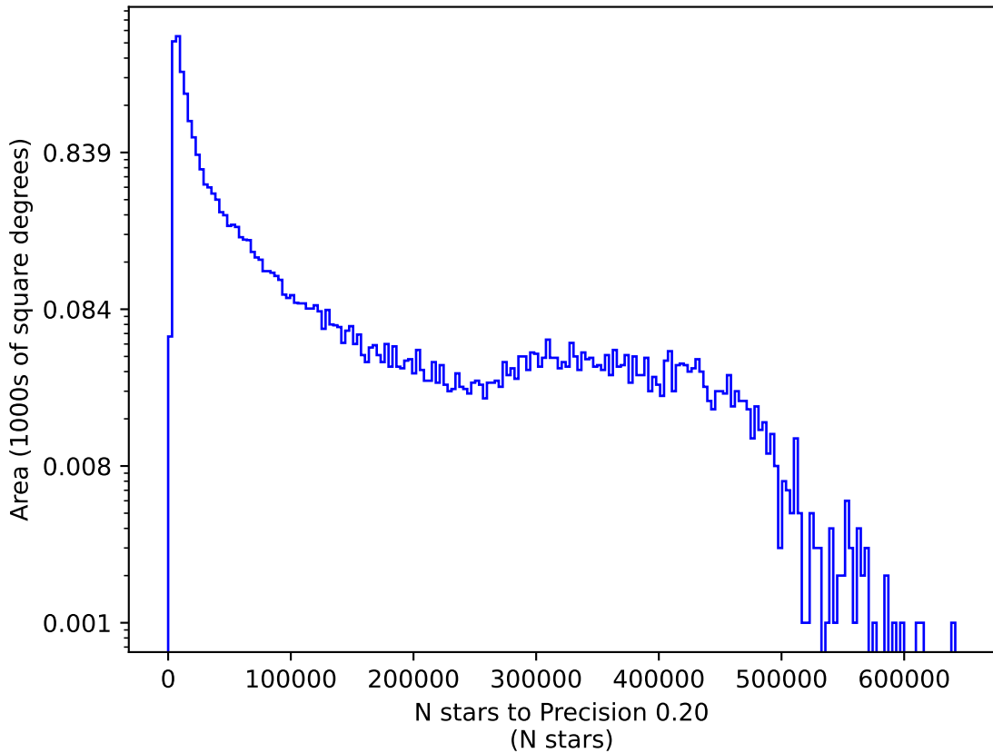
baseline_v3.3_10yrs g: N stars to Precision 0.20
