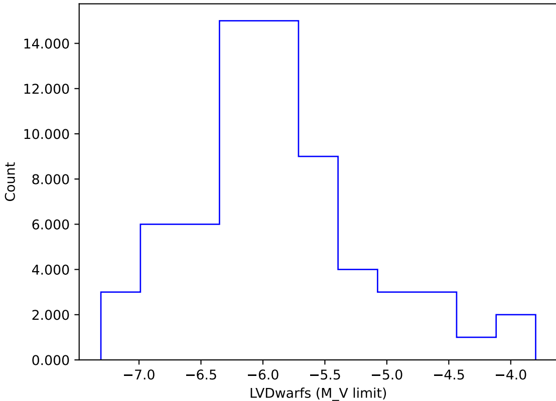
baseline_v3.3_10yrs gi: LVDwarfs
