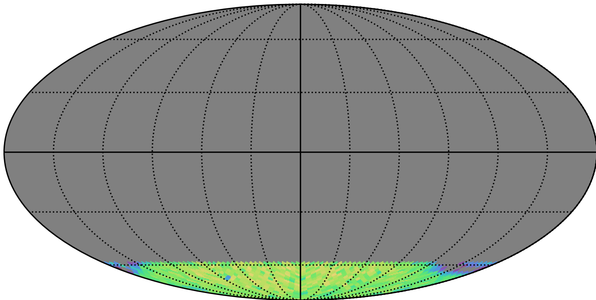
baseline_v3.3_10yrs gi SCP: LVDwarfs
