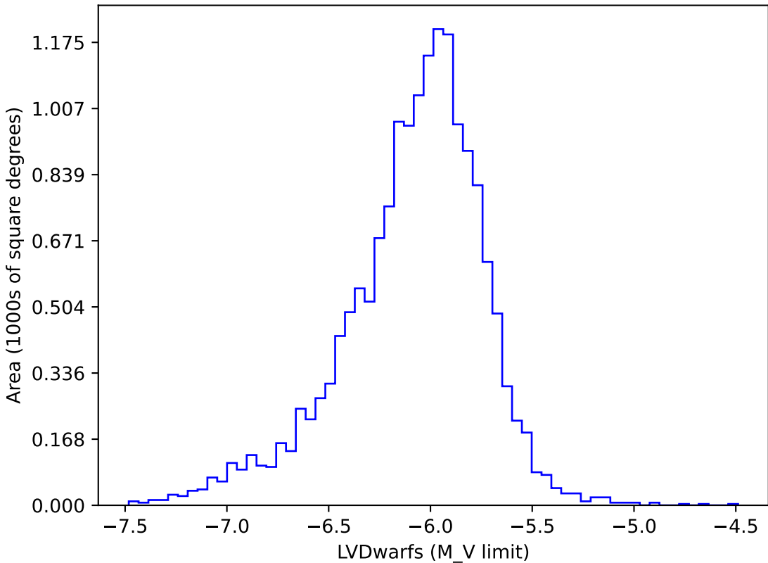
baseline_v3.3_10yrs gi: LVDwarfs
