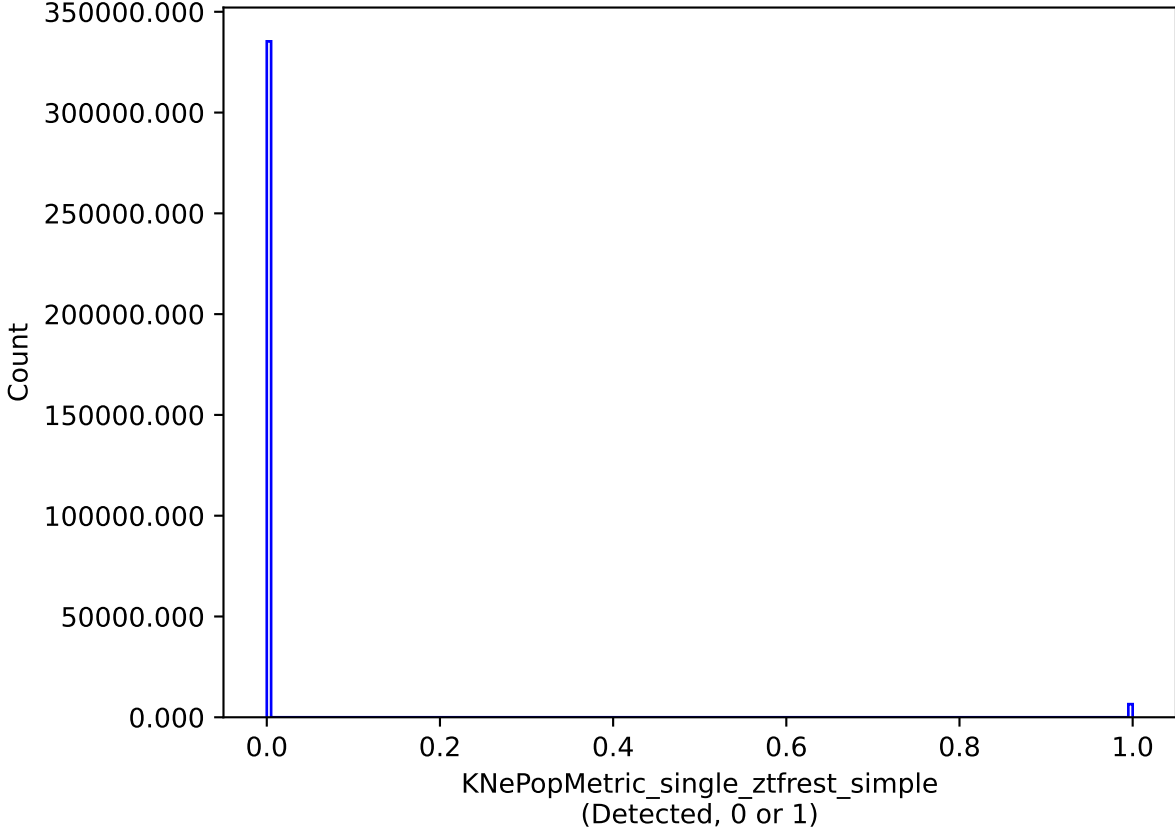
baseline_v3.3_10yrs single model: KNePopMetric_single_ztfrest_simple
