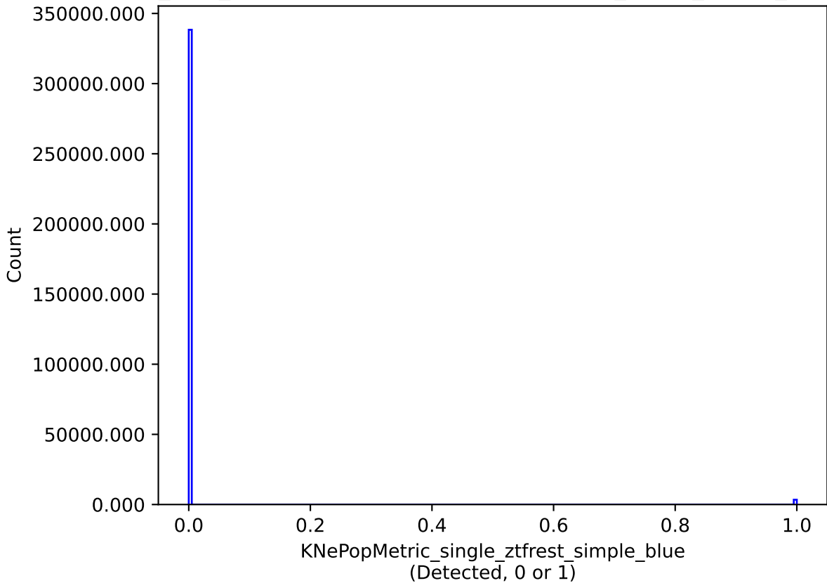
baseline_v3.3_10yrs single model: KNePopMetric_single_ztfrest_simple_blue
