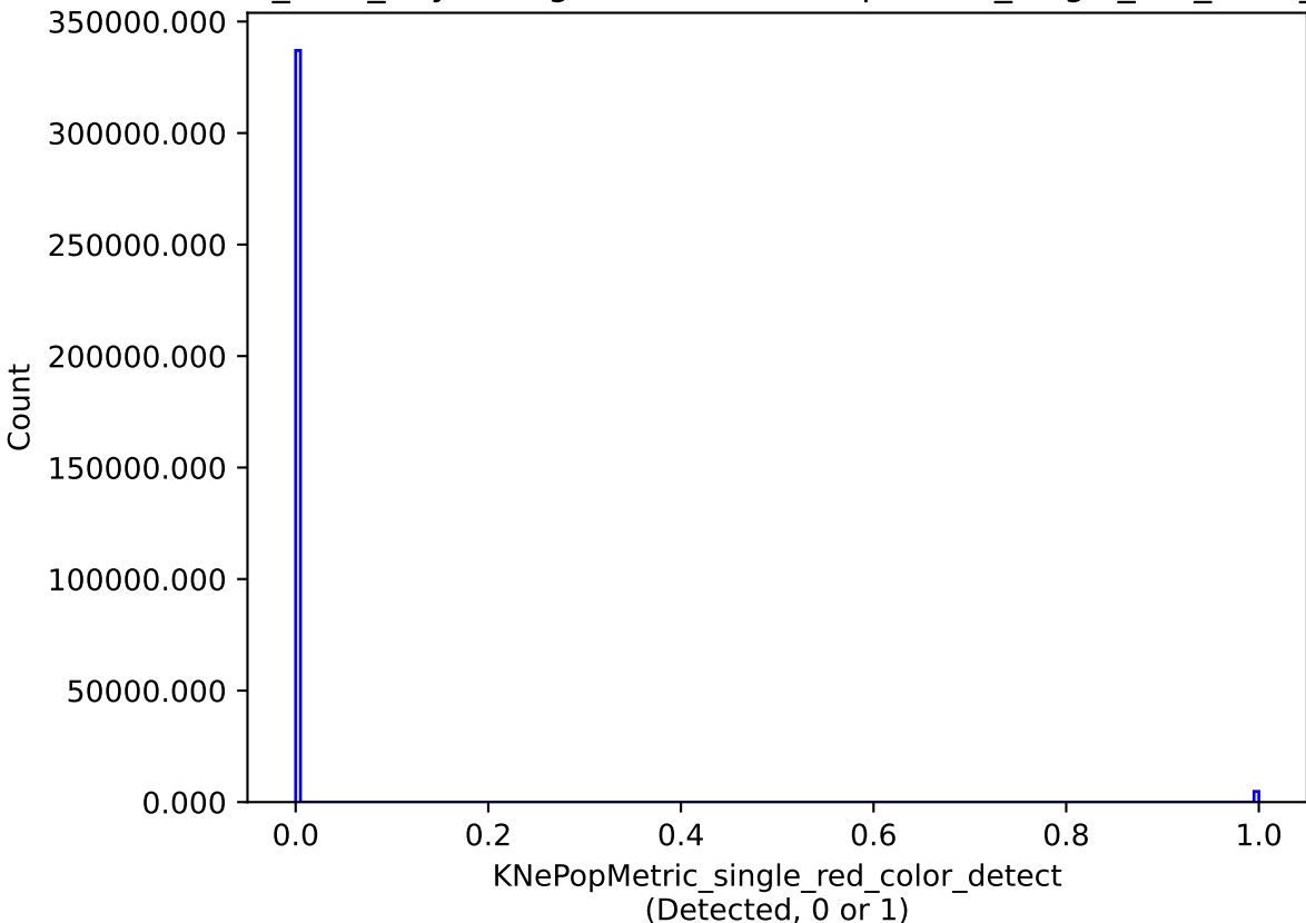
baseline_v3.3_10yrs single model: KNePopMetric_single_red_color_detect
