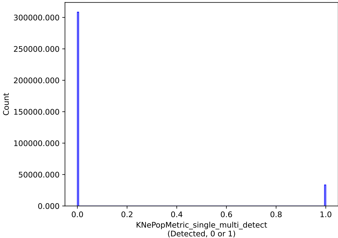
baseline_v3.3_10yrs single model: KNePopMetric_single_multi_detect
