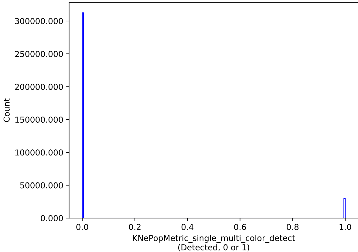
baseline_v3.3_10yrs single model: KNePopMetric_single_multi_color_detect
