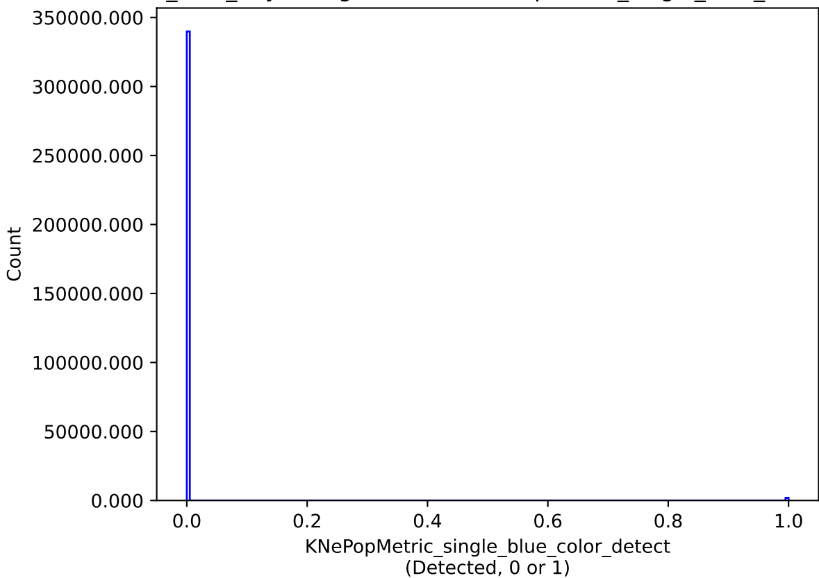
baseline_v3.3_10yrs single model: KNePopMetric_single_blue_color_detect
