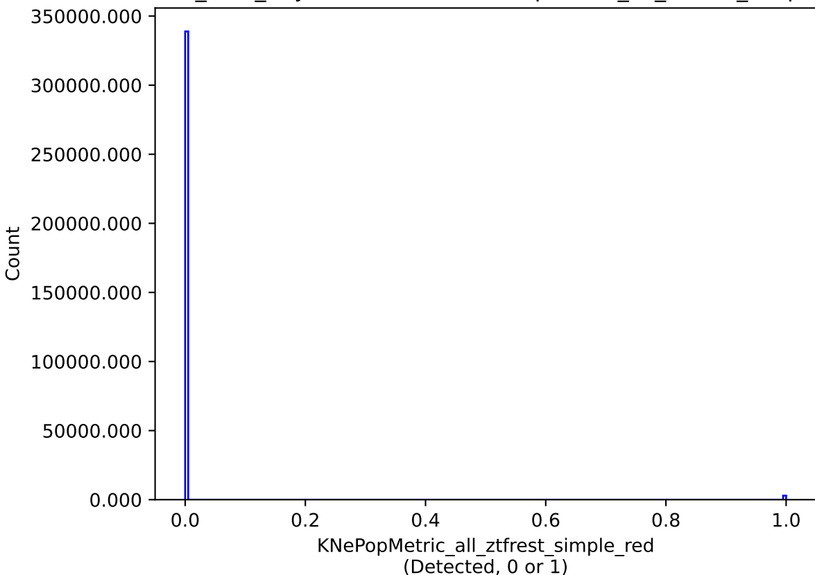
baseline_v3.3_10yrs all models: KNePopMetric_all_ztfrest_simple_red
