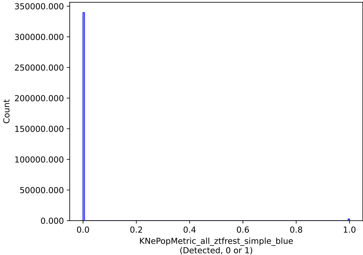
baseline_v3.3_10yrs all models: KNePopMetric_all_ztfrest_simple_blue
