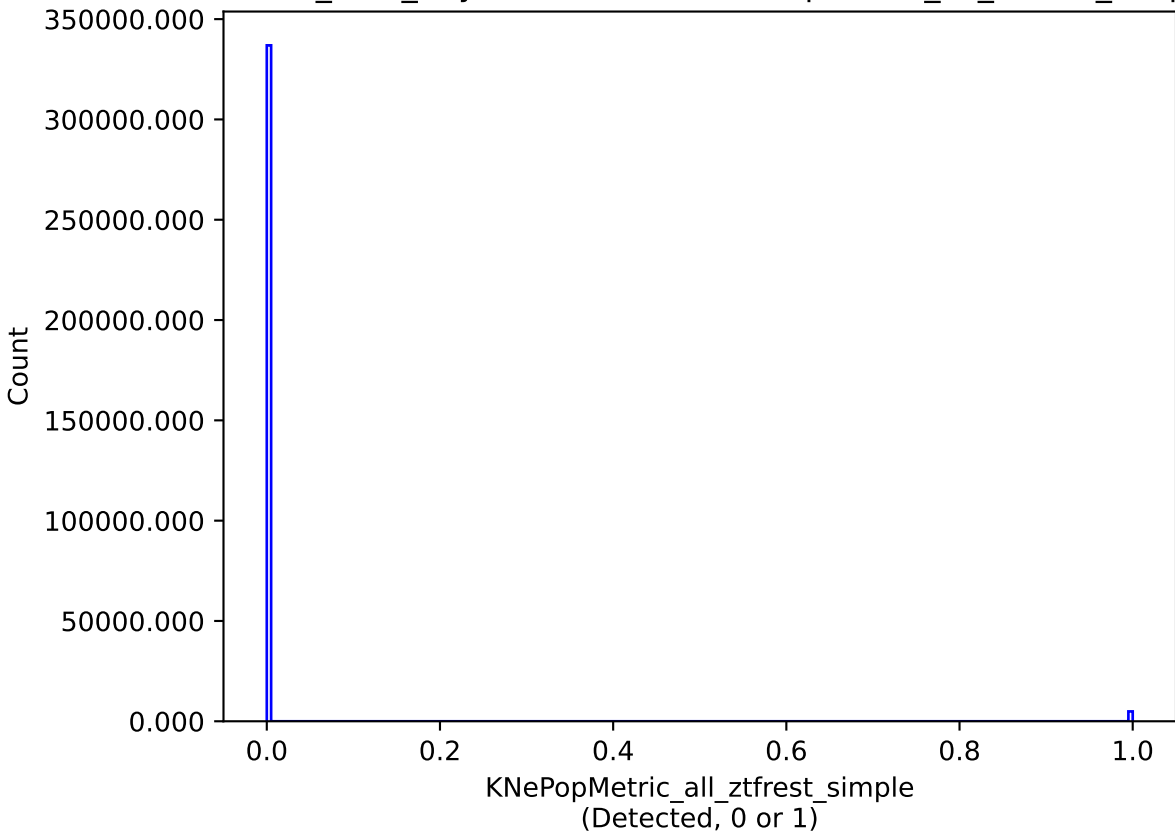
baseline_v3.3_10yrs all models: KNePopMetric_all_ztfrest_simple
