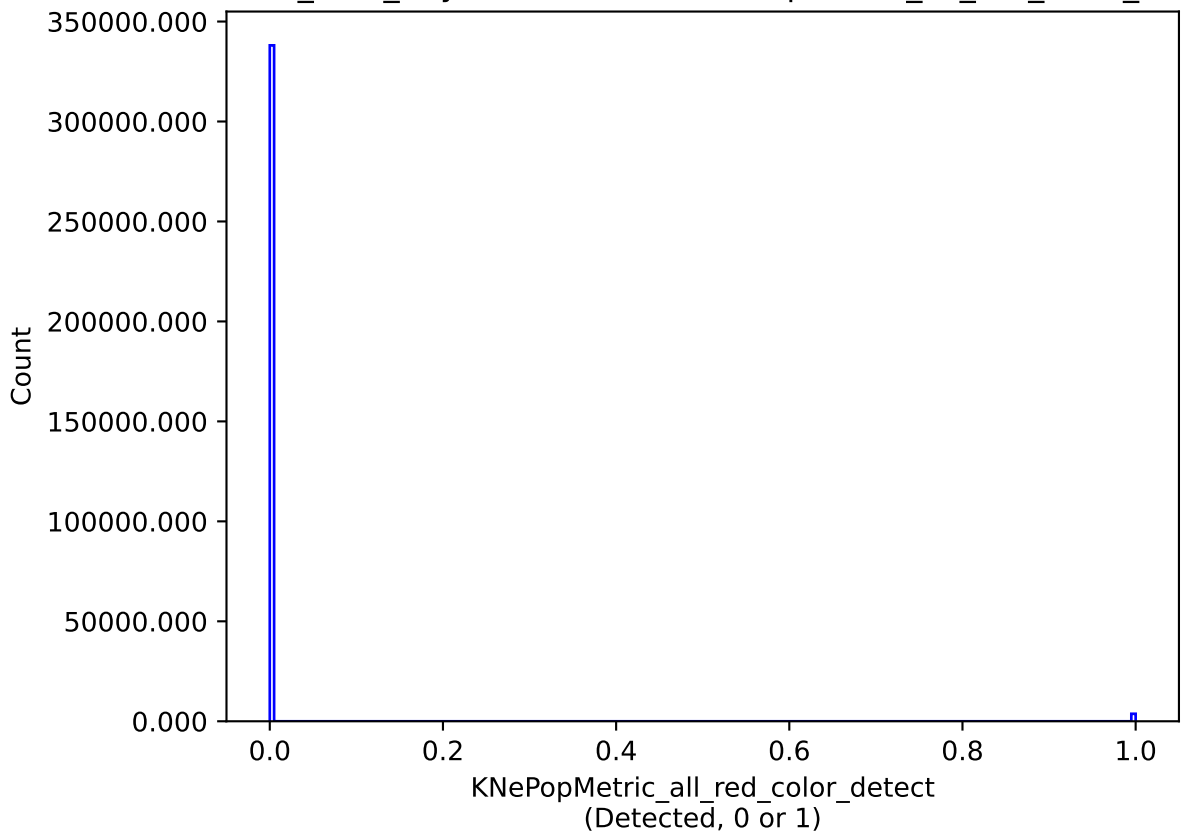
baseline_v3.3_10yrs all models: KNePopMetric_all_red_color_detect
