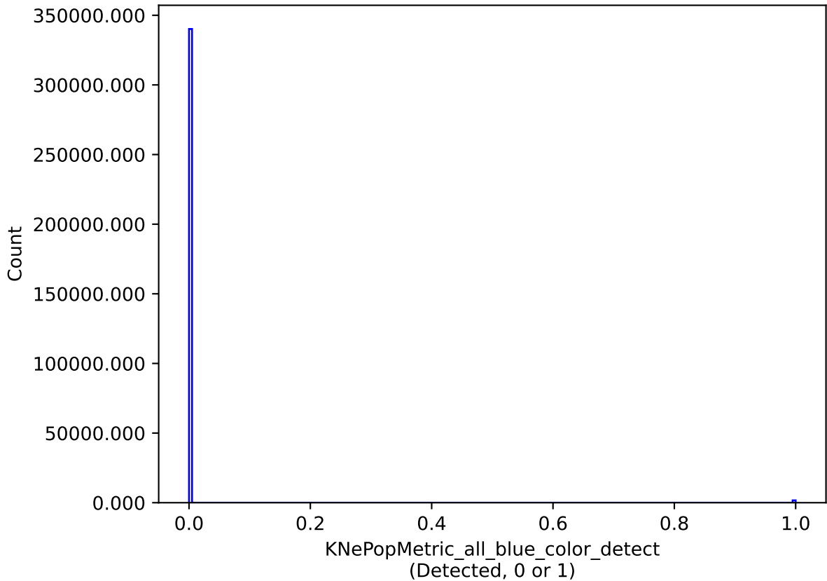
baseline_v3.3_10yrs all models: KNePopMetric_all_blue_color_detect
