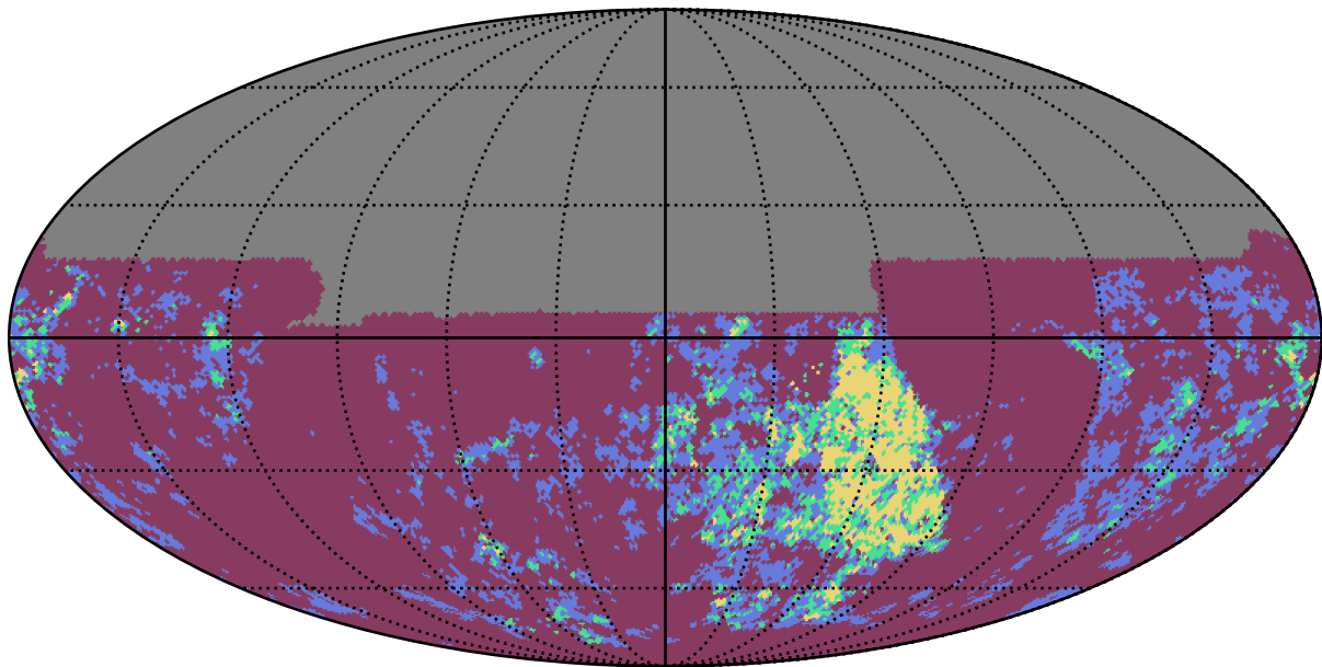
baseline_v3.3_10yrs y band: Gaps_7hr
