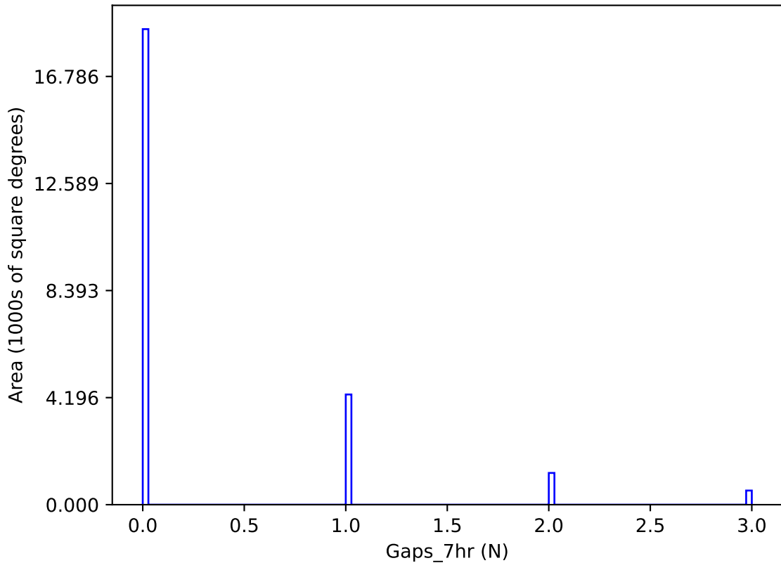
baseline_v3.3_10yrs y band: Gaps_7hr
