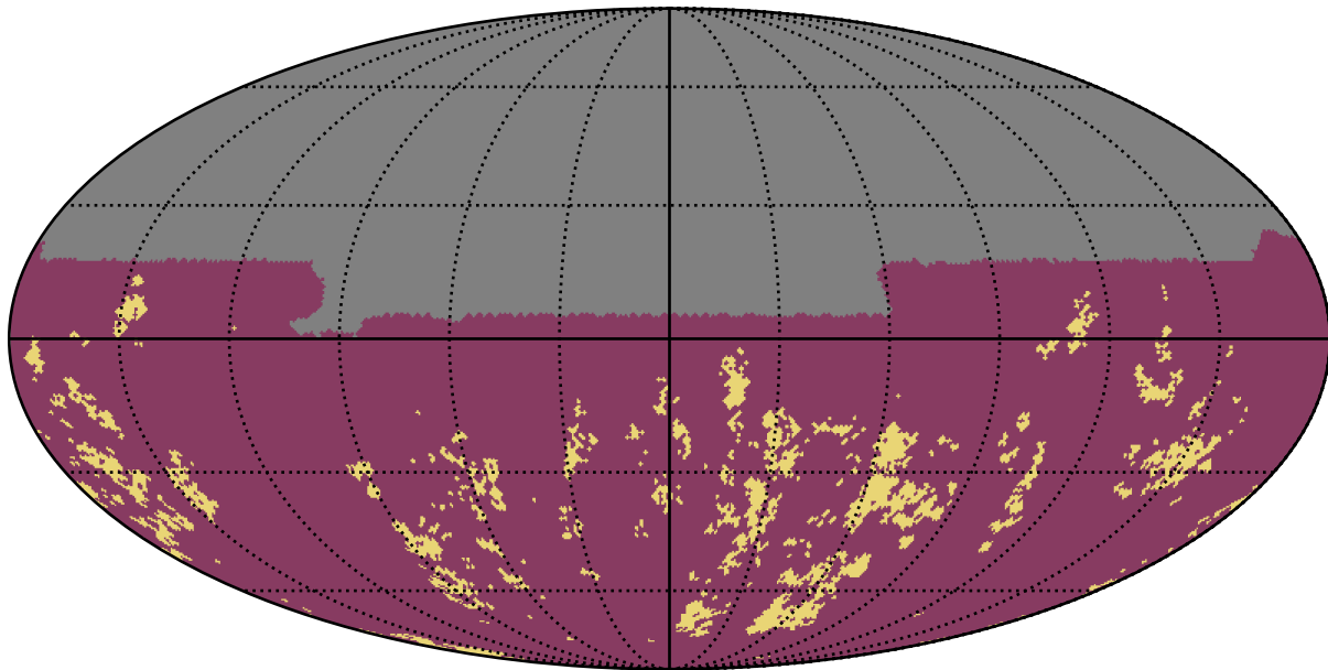
baseline_v3.3_10yrs u band: Gaps_7hr
