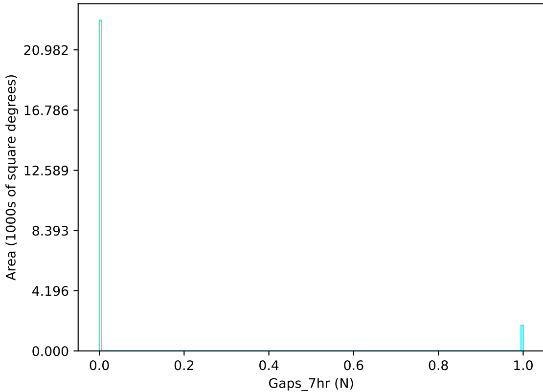
baseline_v3.3_10yrs u band: Gaps_7hr
