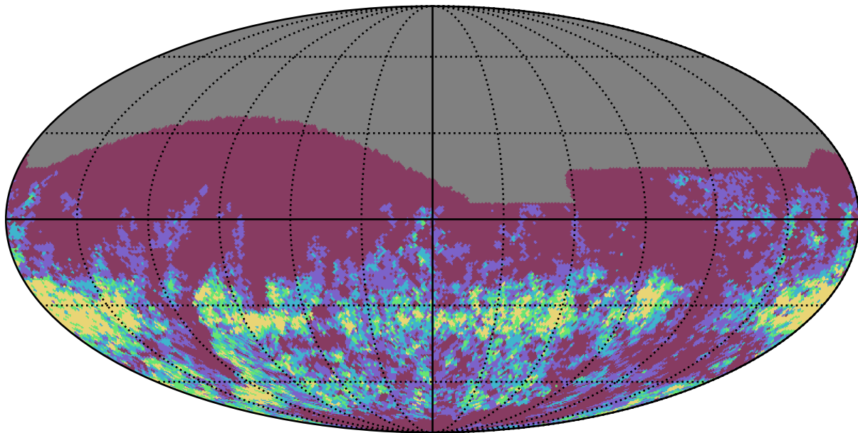
baseline_v3.3_10yrs r band: Gaps_7hr
