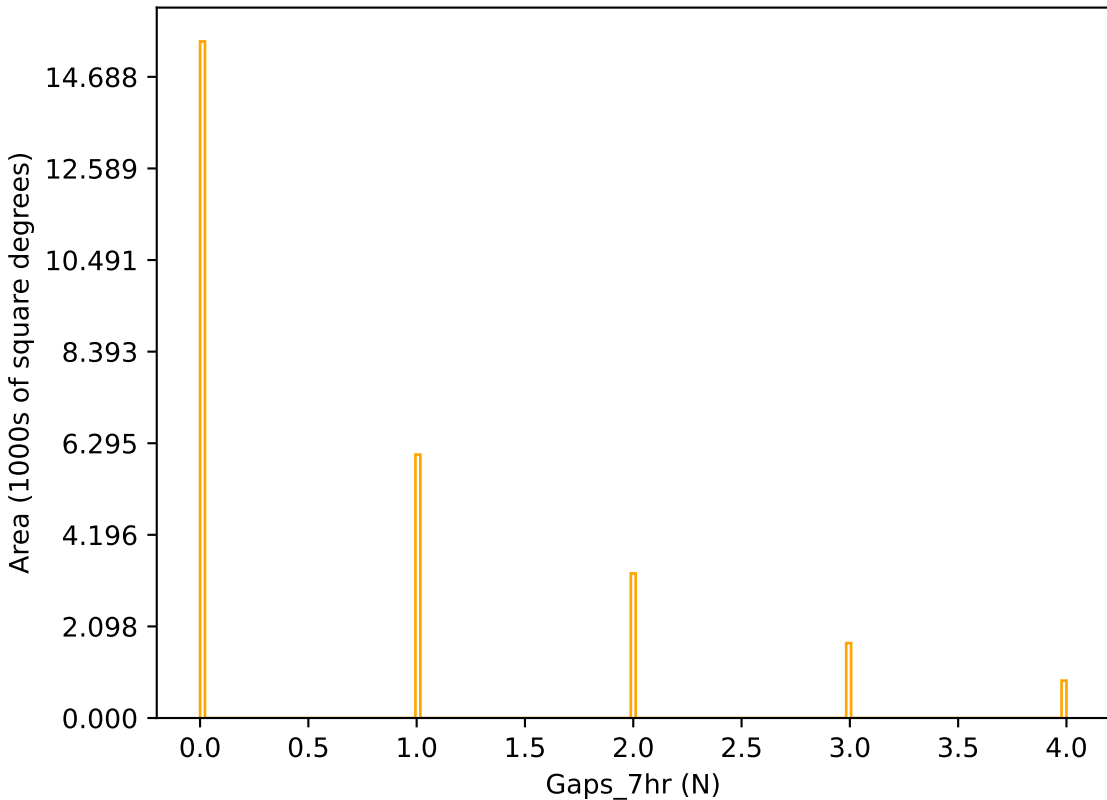
baseline_v3.3_10yrs r band: Gaps_7hr
