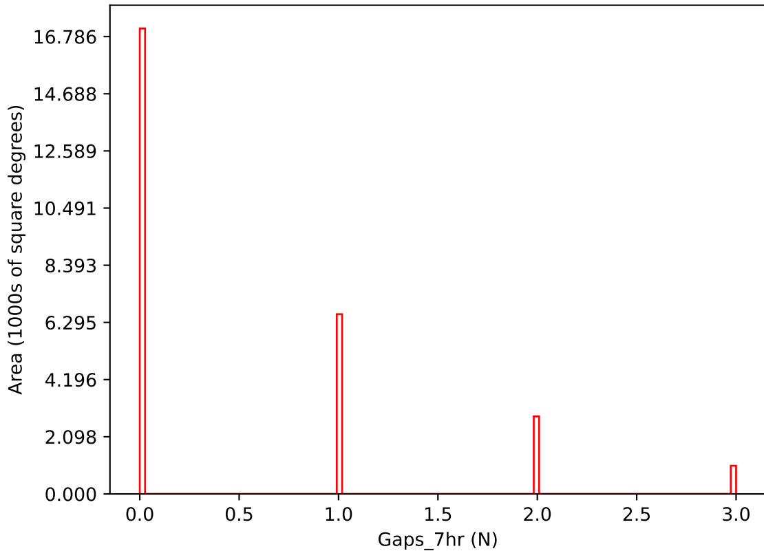
baseline_v3.3_10yrs i band: Gaps_7hr
