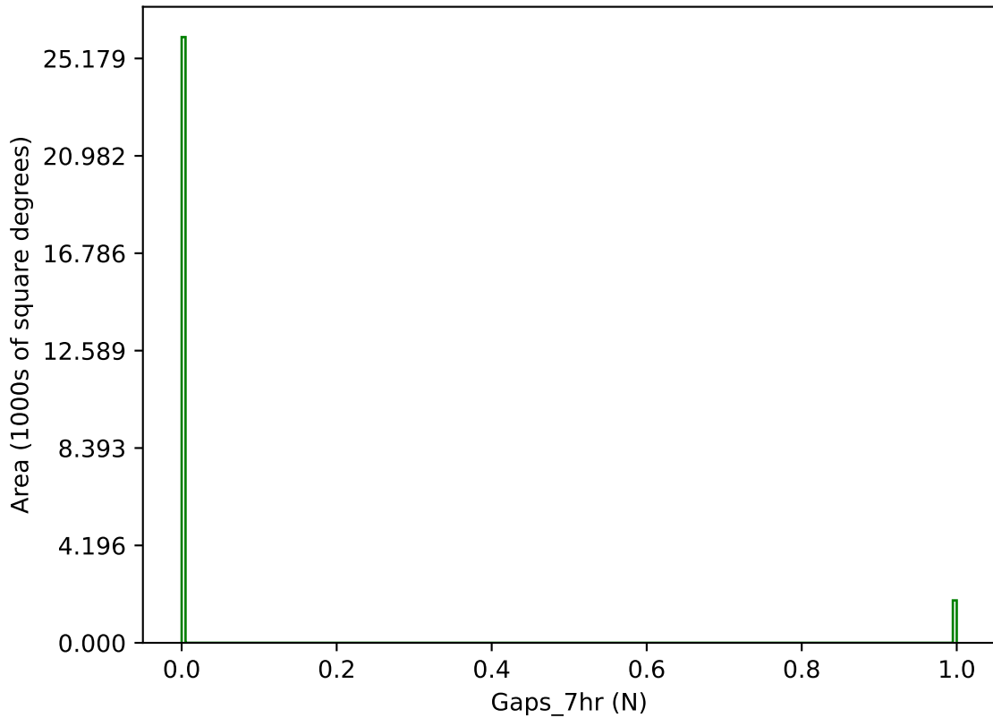
baseline_v3.3_10yrs g band: Gaps_7hr
