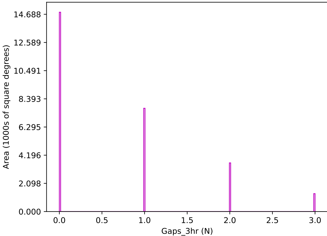
baseline_v3.3_10yrs z band: Gaps_3hr
