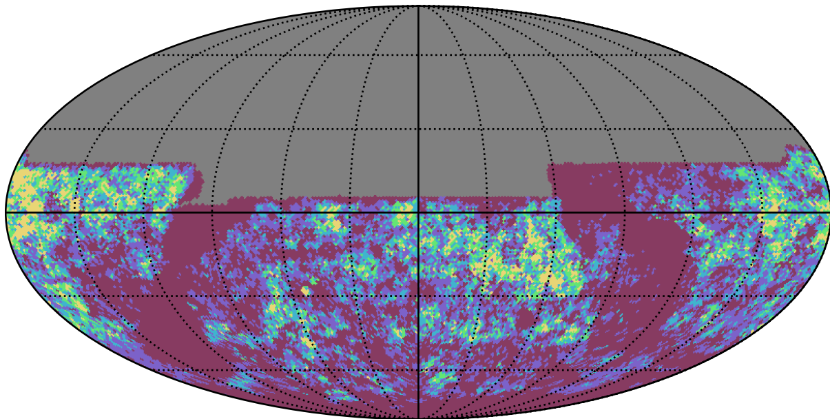
baseline_v3.3_10yrs y band: Gaps_3hr
