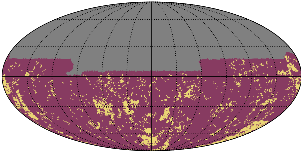
baseline_v3.3_10yrs u band: Gaps_3hr
