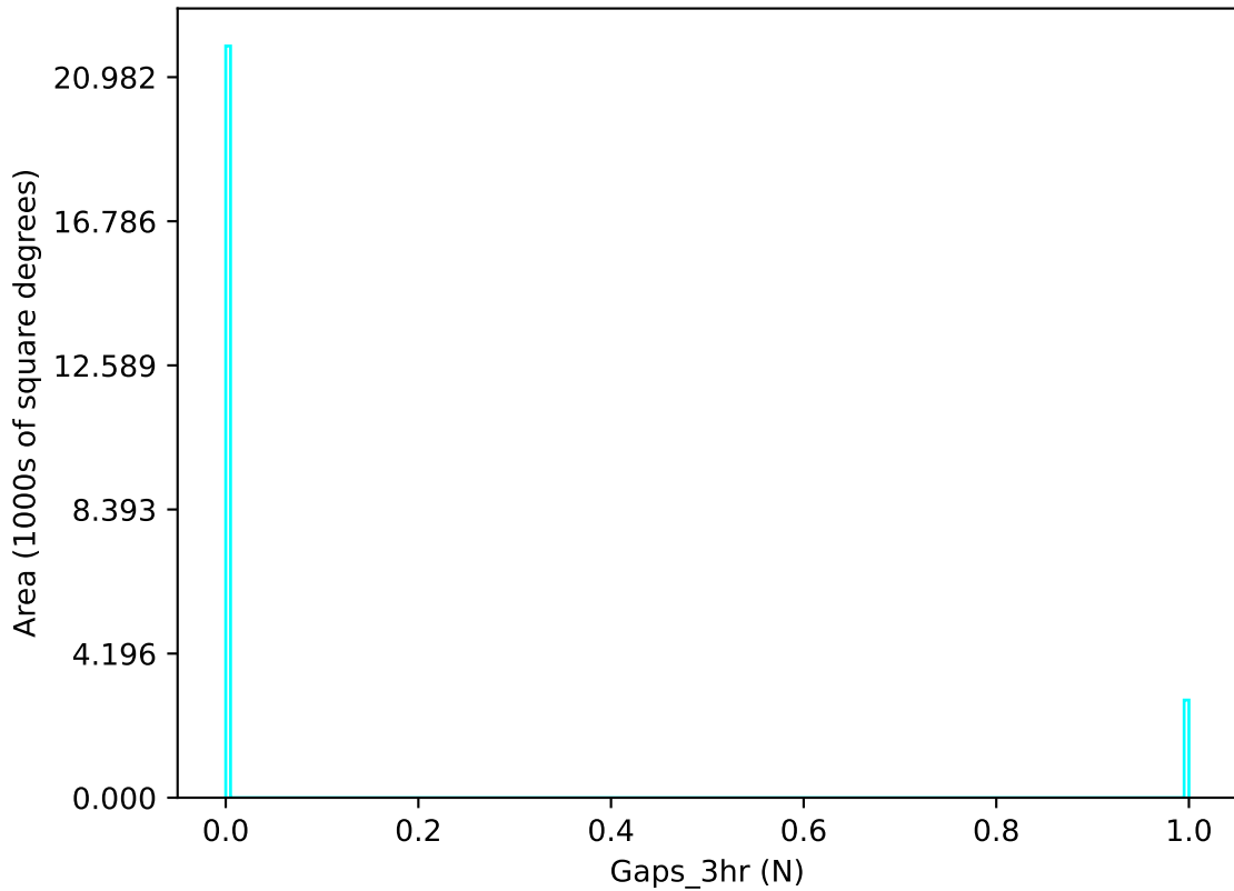
baseline_v3.3_10yrs u band: Gaps_3hr
