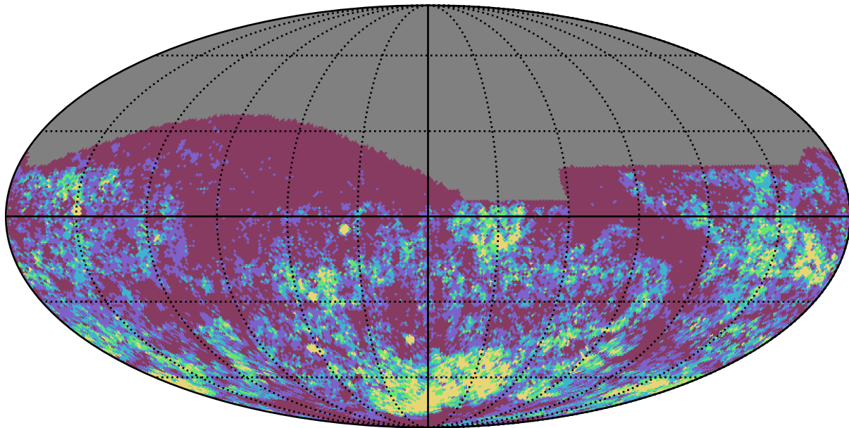
baseline_v3.3_10yrs i band: Gaps_3hr
