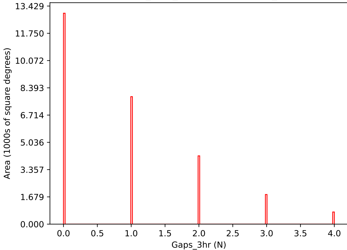
baseline_v3.3_10yrs i band: Gaps_3hr
