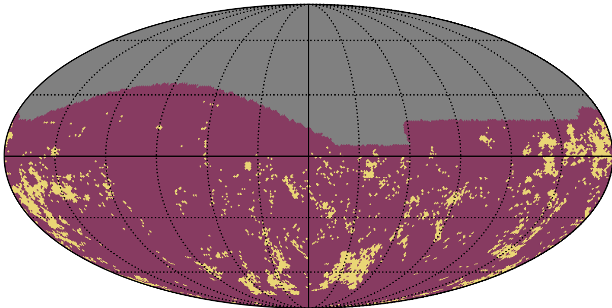
baseline_v3.3_10yrs g band: Gaps_3hr
