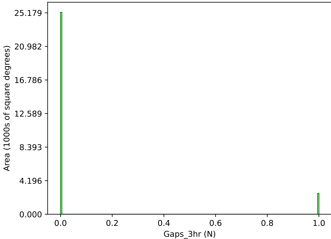
baseline_v3.3_10yrs g band: Gaps_3hr
