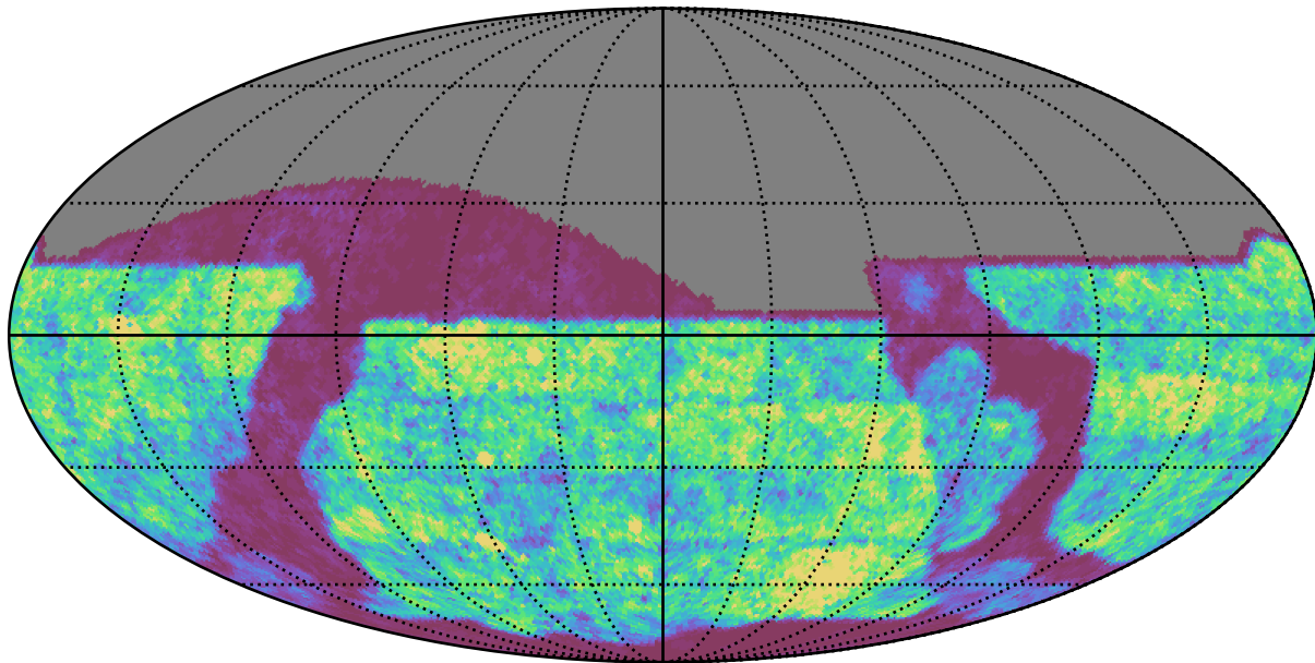
baseline_v3.3_10yrs z band: Gaps_24hr
