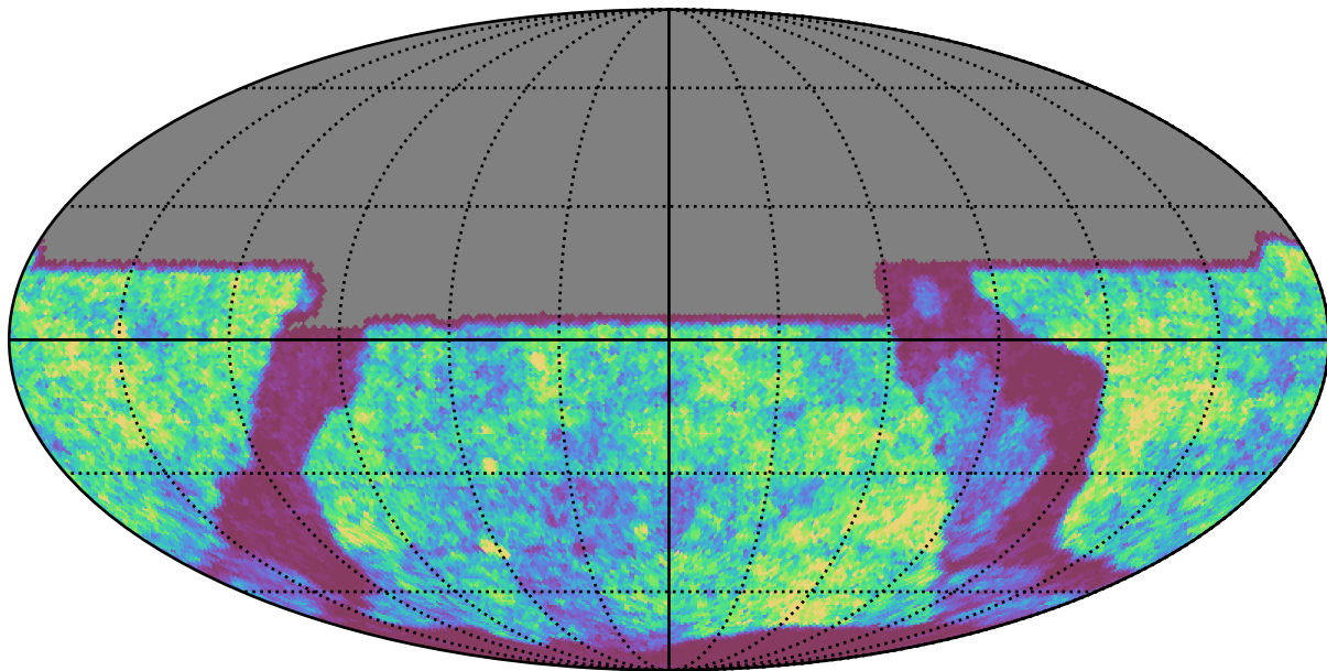
baseline_v3.3_10yrs y band: Gaps_24hr
