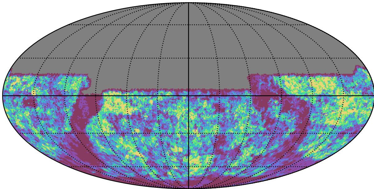
baseline_v3.3_10yrs u band: Gaps_24hr
