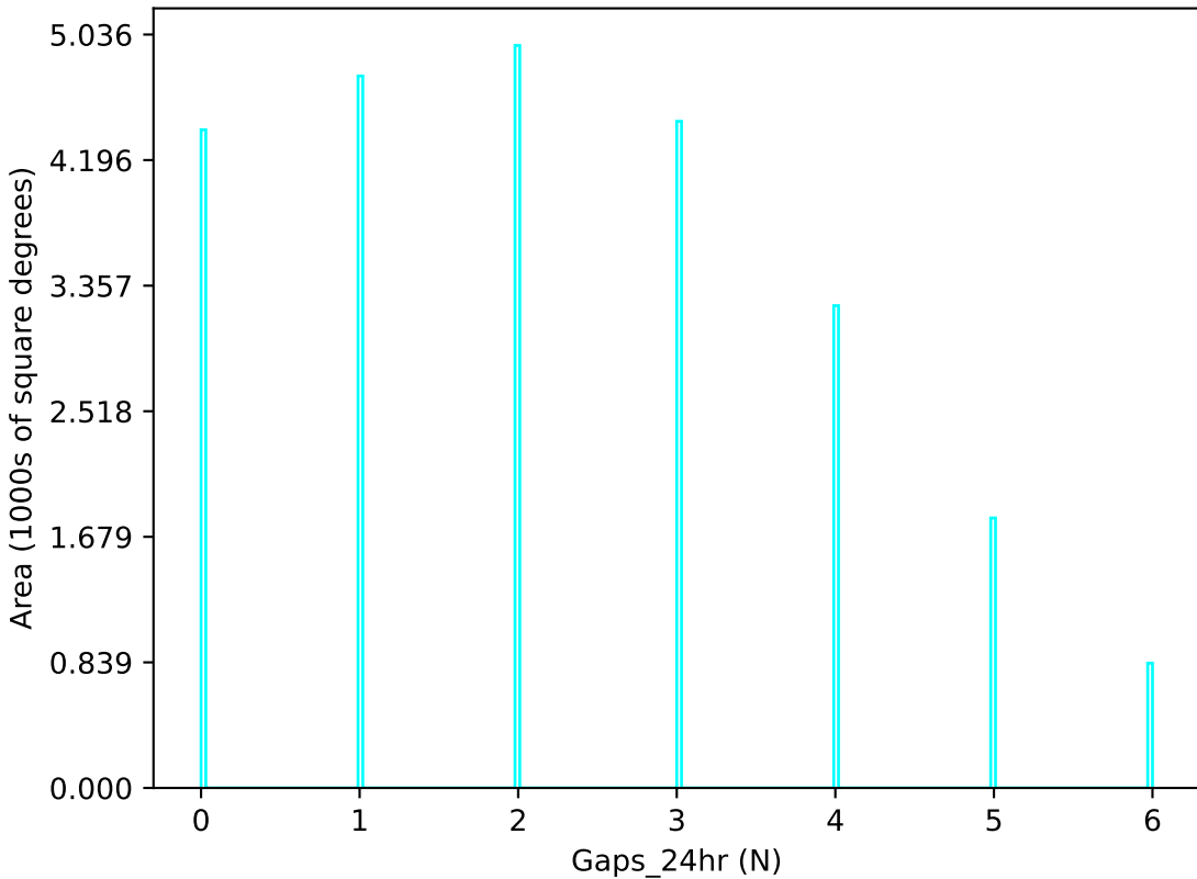
baseline_v3.3_10yrs u band: Gaps_24hr
