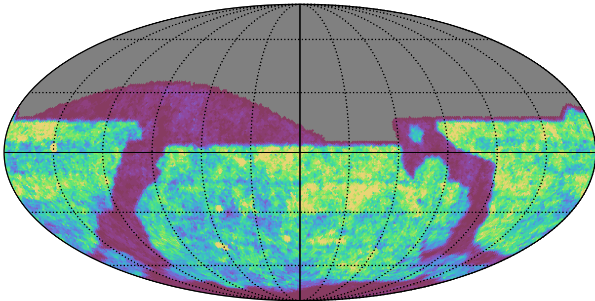
baseline_v3.3_10yrs r band: Gaps_24hr
